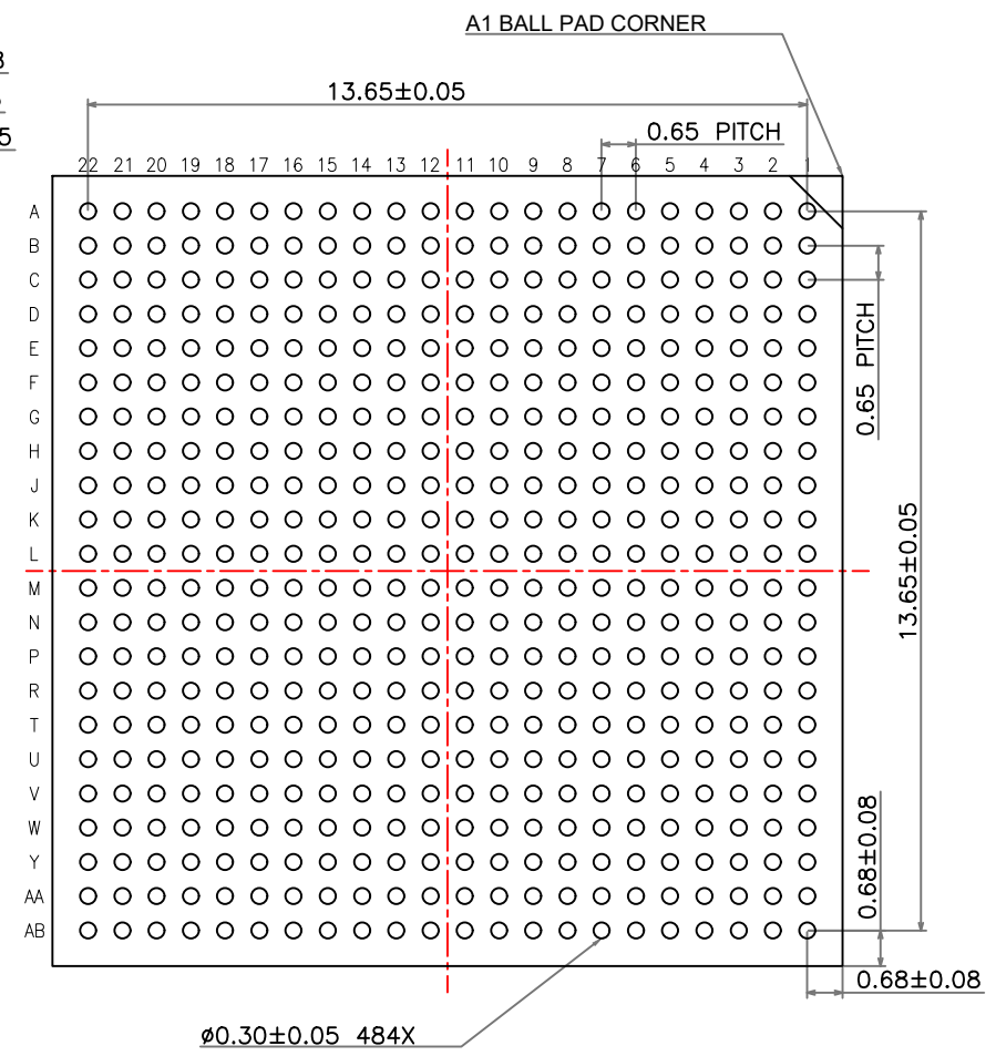
BOTTOM VIEW
